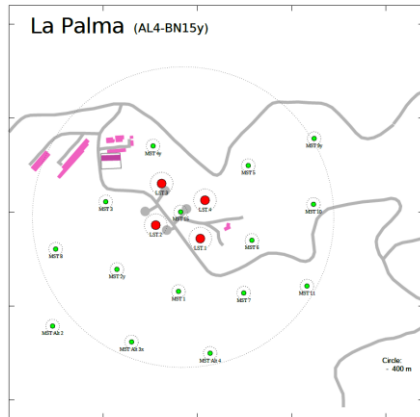
AL4-BN15y layout: 4 LSTs, 15 MSTs
